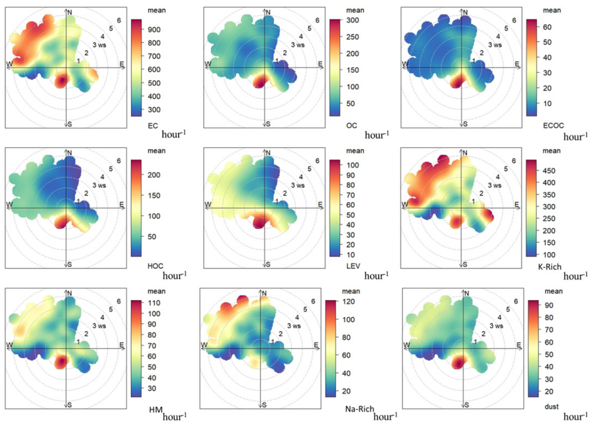
Figure.S2 Polar plots of nine particle types
