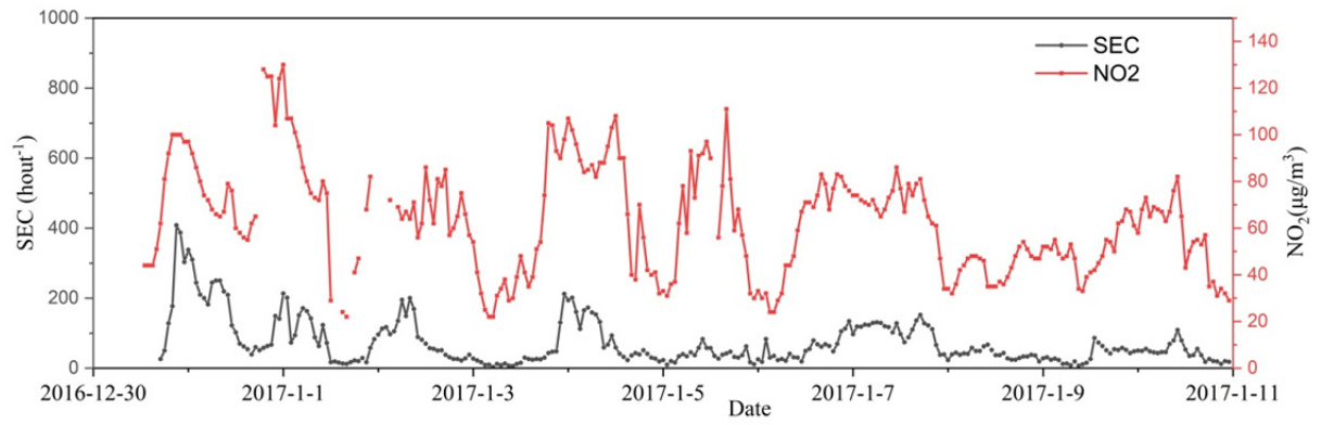
Figure.S1 Temporal profiles of EC particle and NO 2
