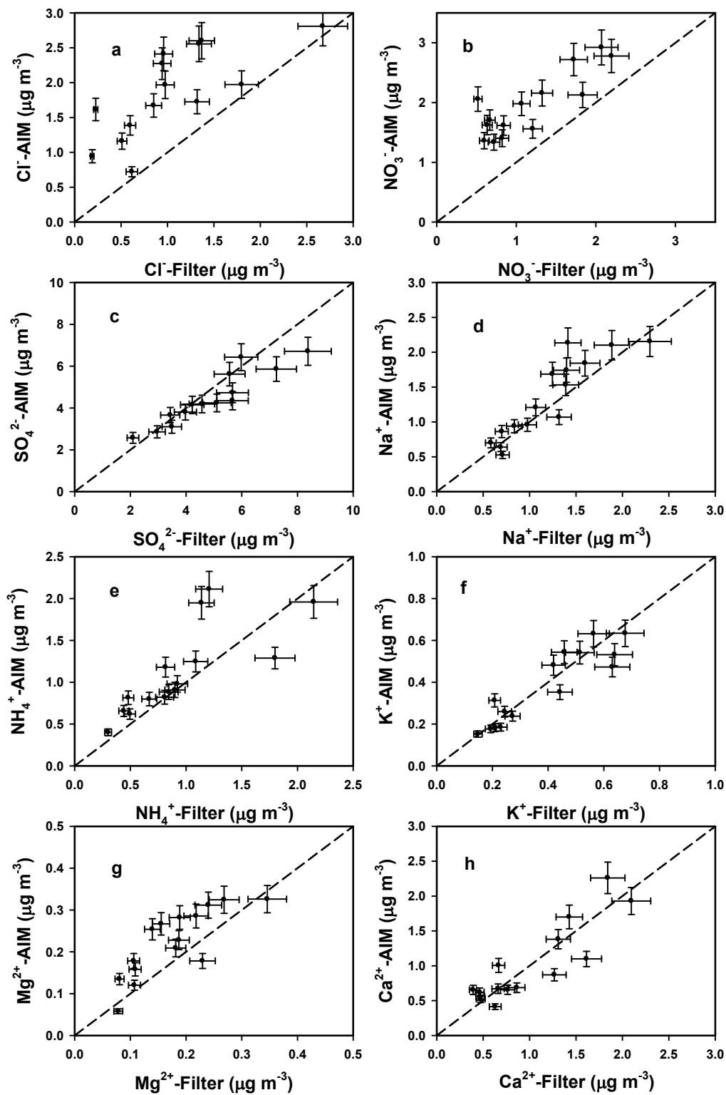
Fig. S1. Scatter plot of measured ionic constituents between the averaged concentration from AIM measurement and filter based measurement. Error bars indicate 10% uncertainty for AIM and filter measurements.
