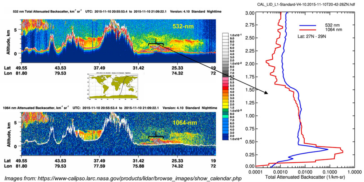
Supp. Figure 1 Curtain plots of CALIOP L1 532-nm (top-left) and 1064-nm (bottom-left) total attenuated back-scatter over northern India for a nighttime overpass of November 10, 2015. (right) A detailed vertical profile of a 2 degrees wide latitudinally averaged attenuated back-scatter for both wavelengths.
