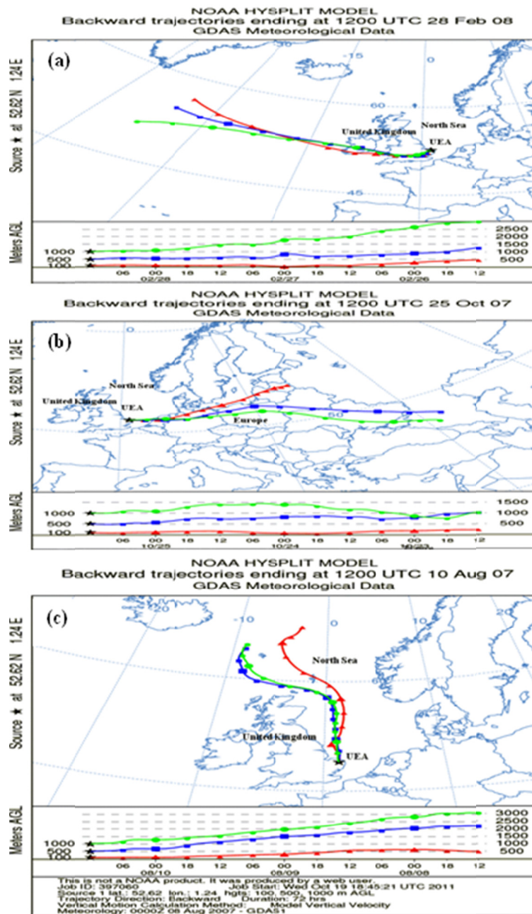
Fig. S1. Example of trajectories. Result of the HYSPLIT model 3-day backward trajectory analysis started at 1200UTC, at altitudes of 100, 500 and 1000 m at UEA station. The top and bottom panels display horizontal and vertical motion. Symbols denote the location of the air parcel every 6 hours.
