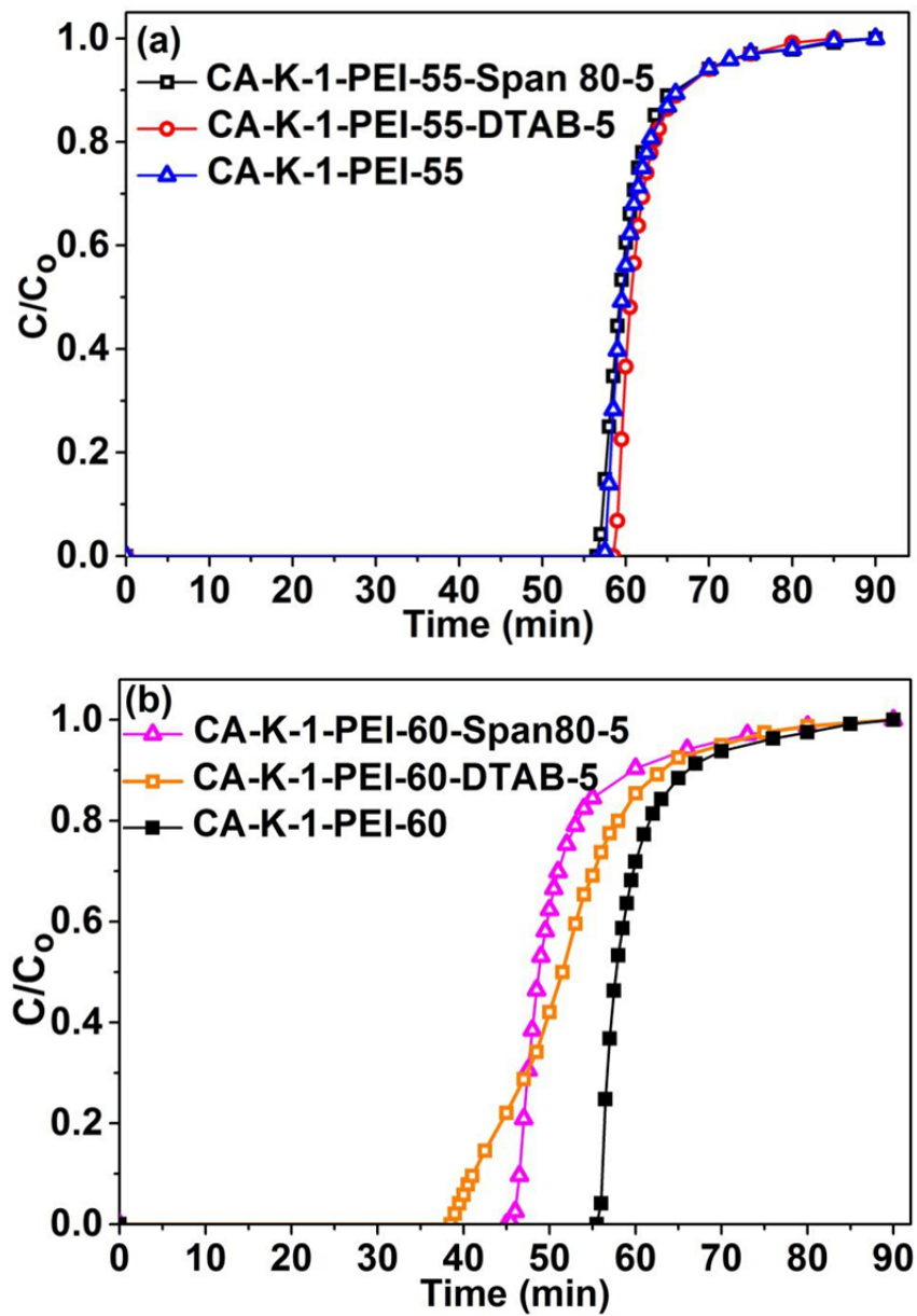
Fig. S1. CO 2 adsorption breakthrough curves of PEI-loaded CA-K-1 with and without surfactants addition.
