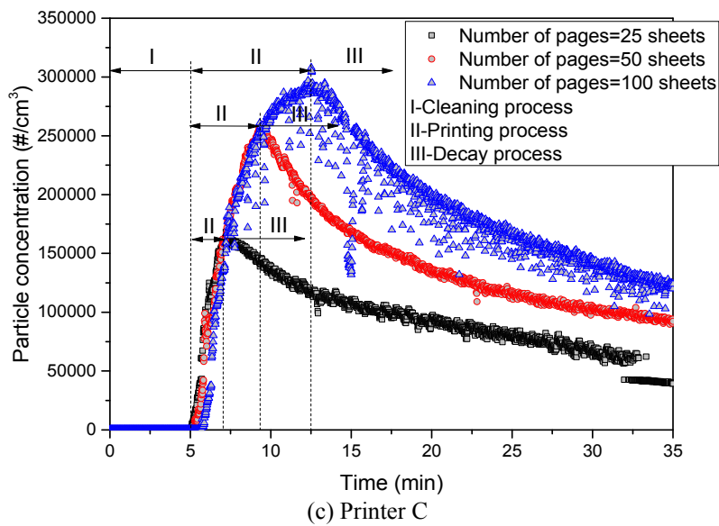
Fig. 5. Effect of number of pages on real-time ultrafine particle emissions.
