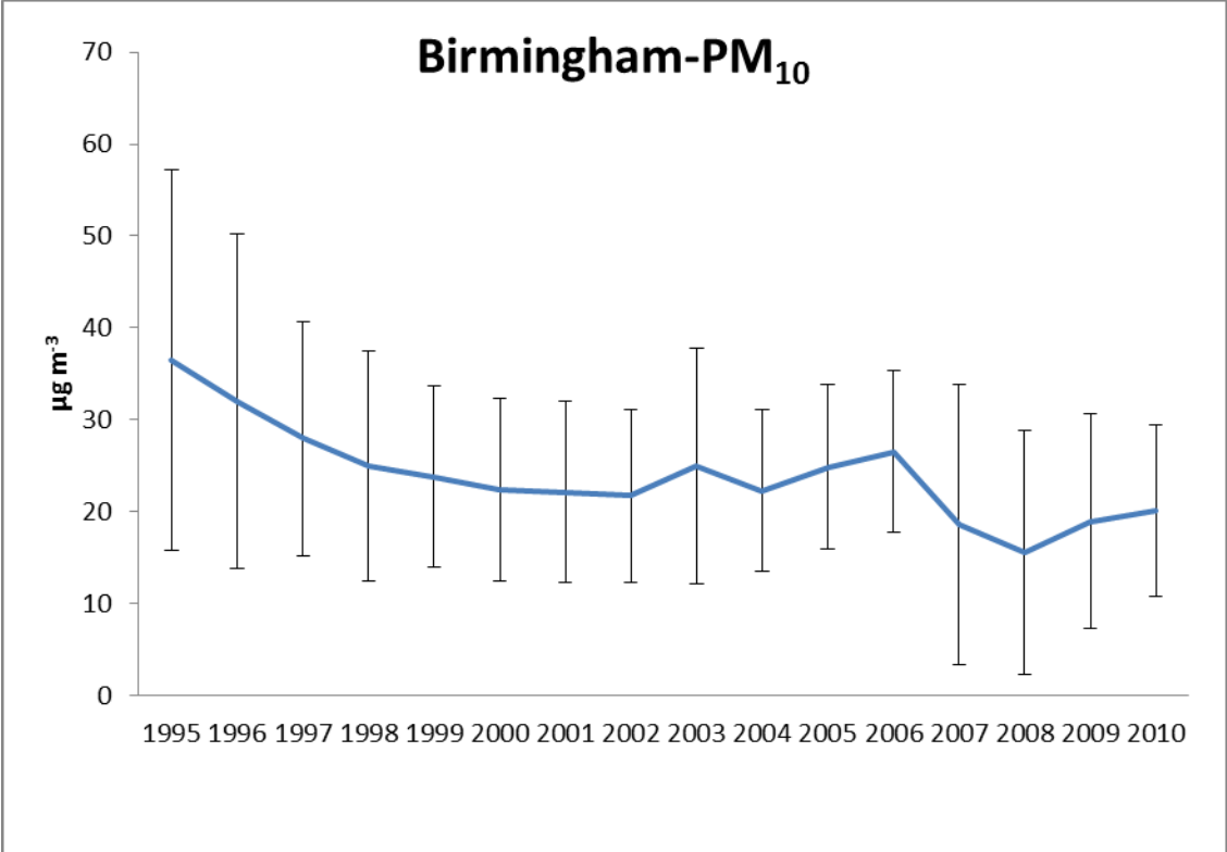
Figure S1: Annual PM 10 data for Birmingham between 1995 and 2010 (Data from the Birmingham City Center (1995 to 2008) and Birmingham Tyburn Roadside's (2009-2010) Automatic Urban Rural Network (AURN) Site at uk-air.defra.gov.uk/networks/aurn-site-info )
