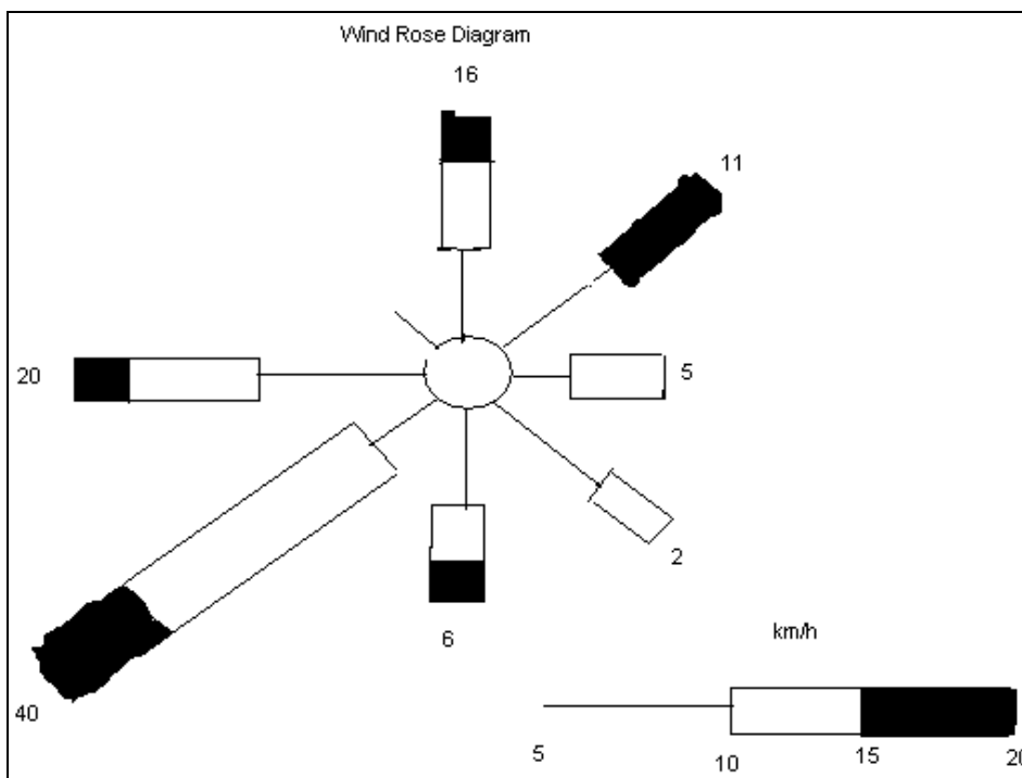
Fig. 2. Wind rose diagram in Raipur during the study period (Wind speed in km/h).
