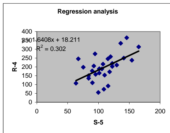
Fig. 3(d). Regression graph of source-receptor ambient PM 10 levels monitored in an urban area for receptor site R-4.
