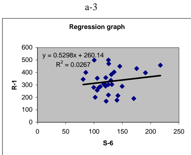
Fig. 3(a). Regression graph of source-receptor ambient PM 10 levels monitored in an urban area for receptor site R-1.
