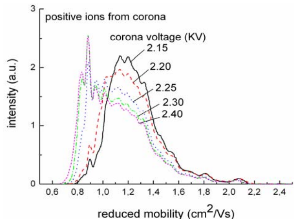
Fig. 7. Mobility spectra of positive air ions as a function of the corona voltage.
