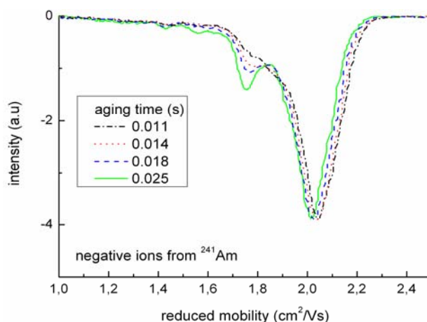
Fig. 3. Evolution of the mobility distribution of negative air ions generated by ^{241}\text{Am} during the early stages of aging.
