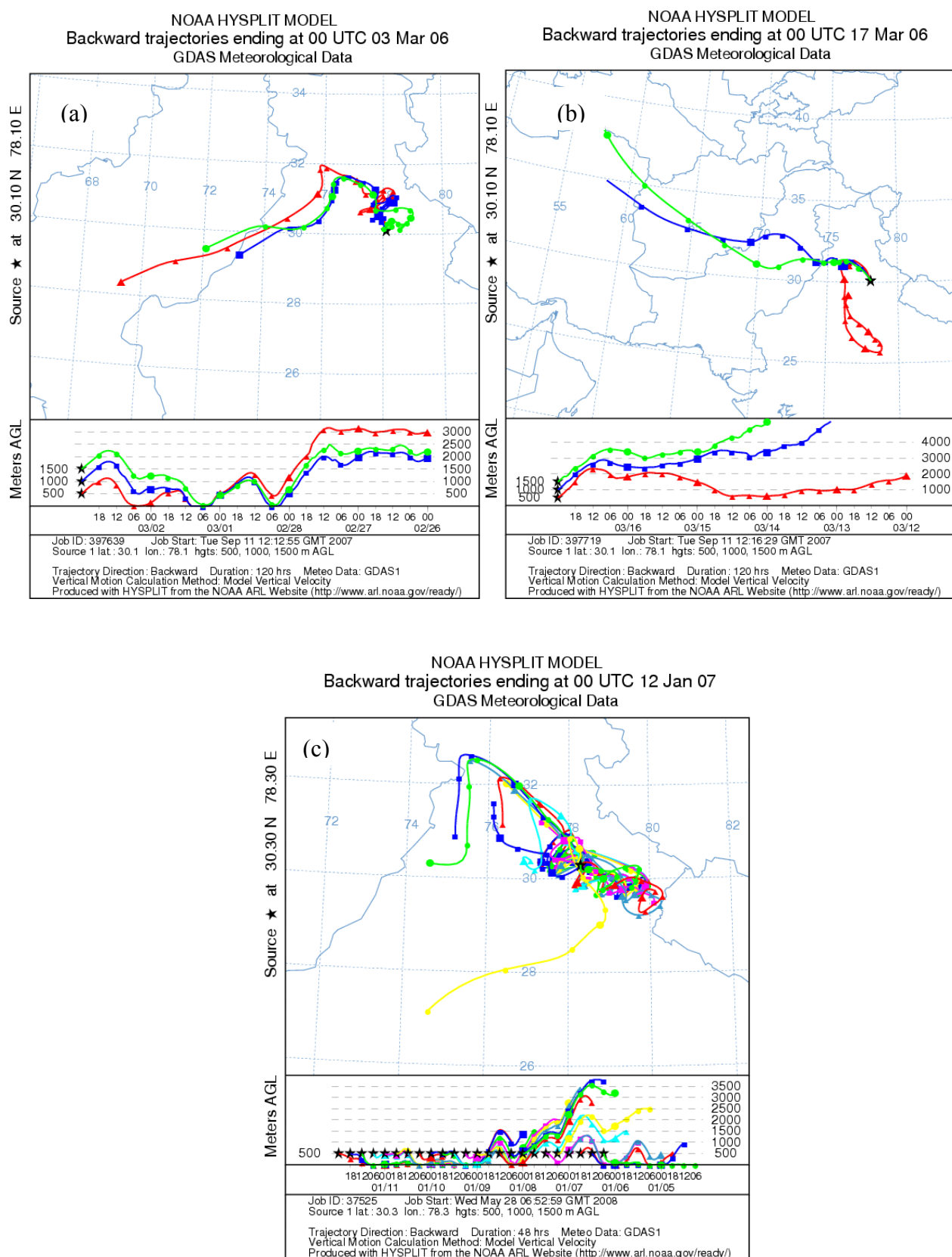
Fig. 5. NOAA-HYSPLIT model trajectory map during clear and turbid days of March 2006 and January 2007.
