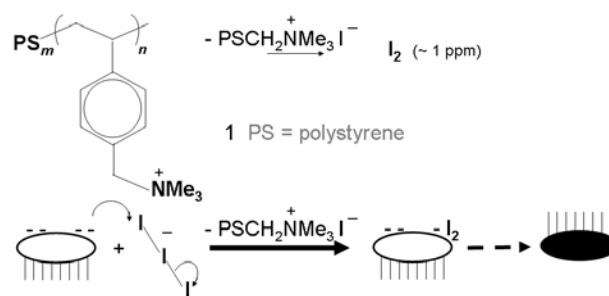
Fig. 1. Poly(styrene–divinylbenzene)-4-(trimethylammonium)methyl triiodide (1) and its conceptual mechanism for disinfecting microorganisms.
