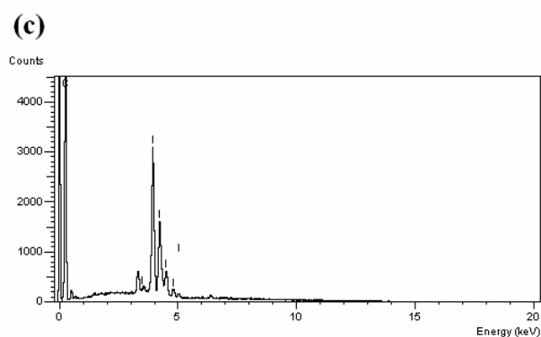
Fig. 3. (a) SEM image of untreated filter at 700X; (b) SEM image of enlarged fleck at 2500X; (c) EDX spectrum of (b).
