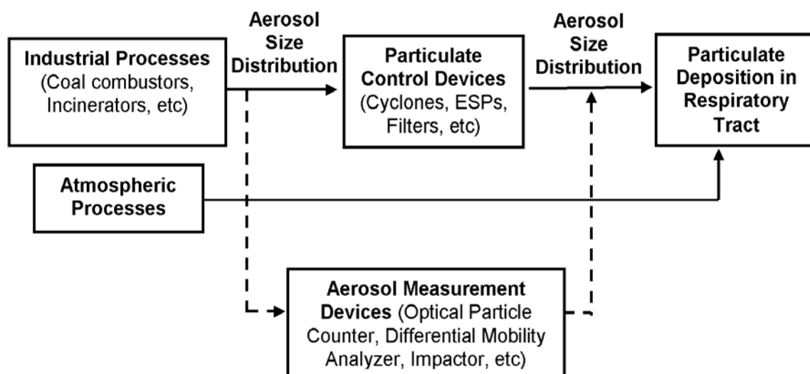
Fig. 1. Algorithm chart of the web-based aerosol program.
