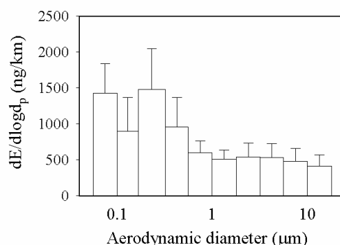
Figure 3. Size distributions of sum of 20 PAHs in motorcycle exhaust.
