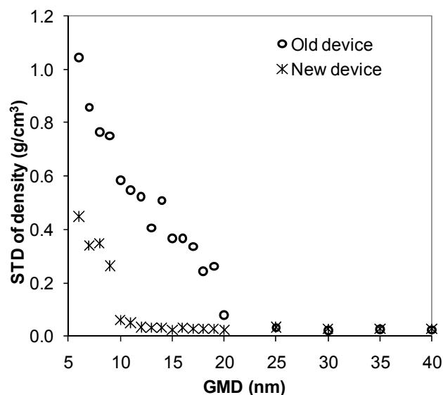
Fig. 5. The result of the simulation. STD of density results increases as mode GMD decreases. The Deviation of the old (open circles) and the new impactor device (black stars) start to increase after 20 nm and 10 nm, respectively.
