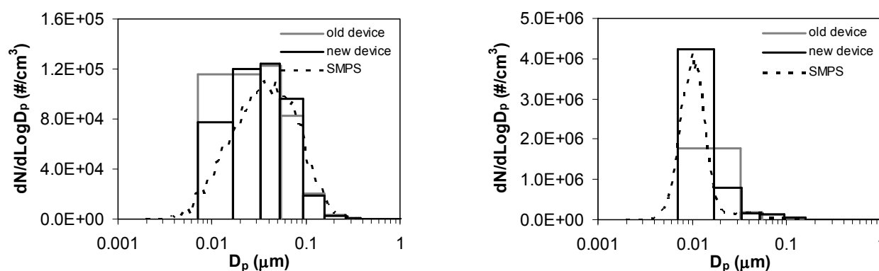
Fig. 3. Examples of the size distributions measured with different devices from Euro IV compliant medium duty diesel engine exhaust. The engine was tested in different points of European Stationary Cycle (ESC). Results from ESC11 (left) and ESC10 (right) are shown in the figure.
