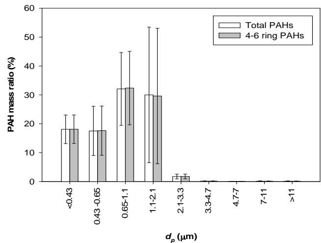
Fig. 11. Size distributions of total and 4–6 ring PAHs in terms of mass ratio.
