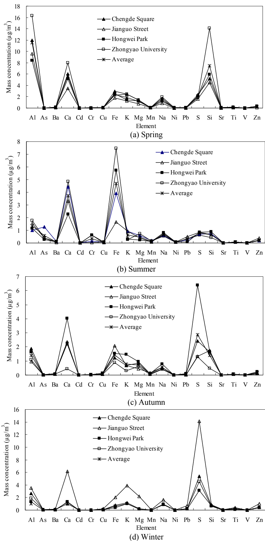
Fig. 3. Elemental concentrations of PM 10 at four sites during four seasons in Harbin, China.
